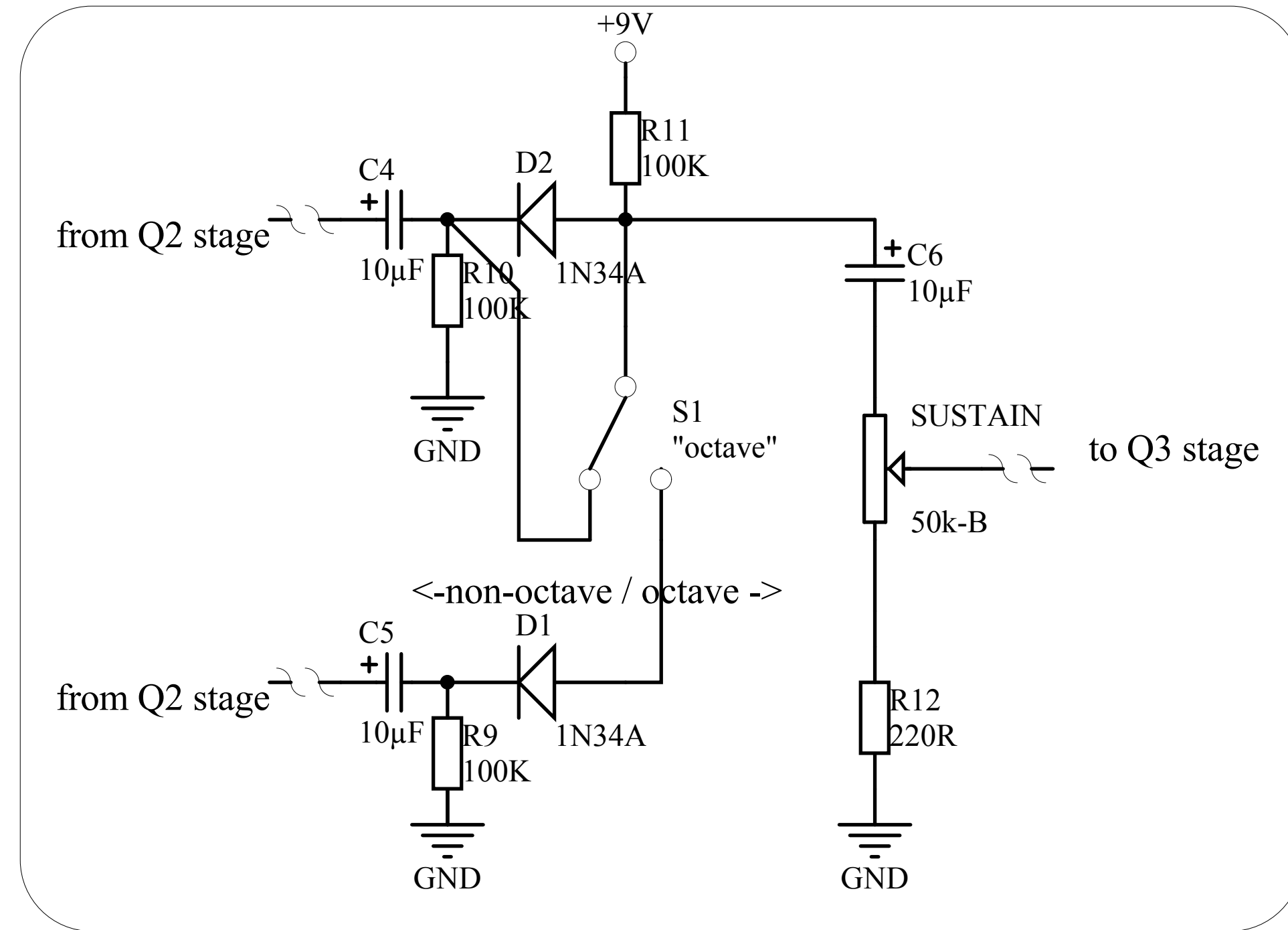
improved FTM octave switch wiring as suggested by Mark Hammer of diystompboxes.com
