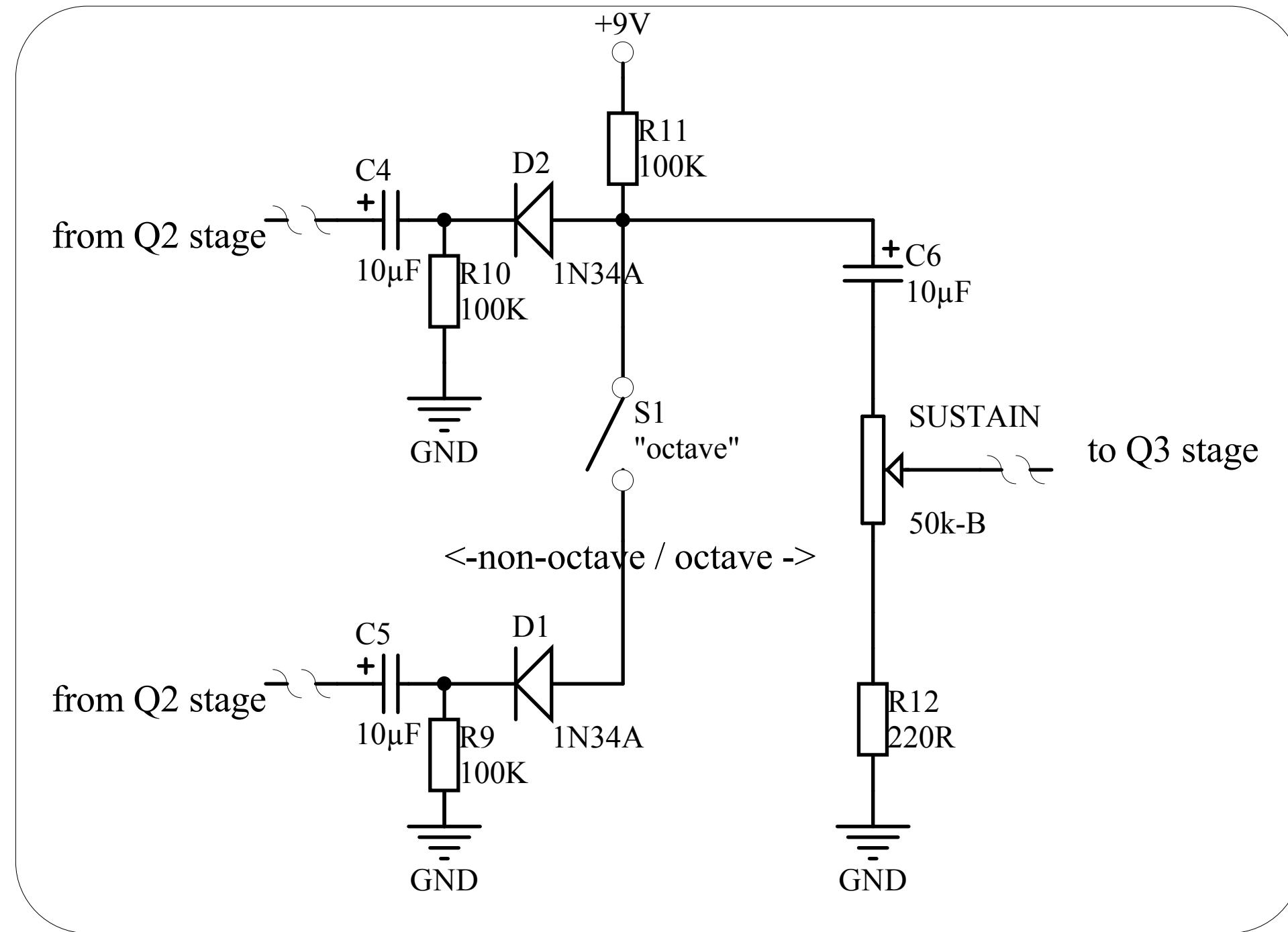
stock FTM octave switch wiring
